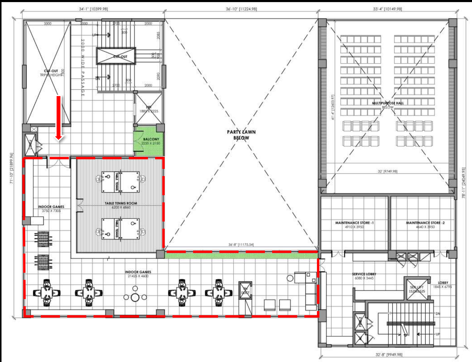
First Floor Plan – Indoor games
