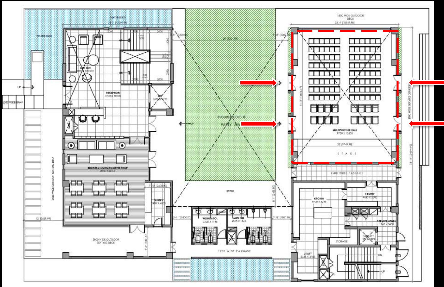
Ground Floor Plan – Multipurpose Hall
