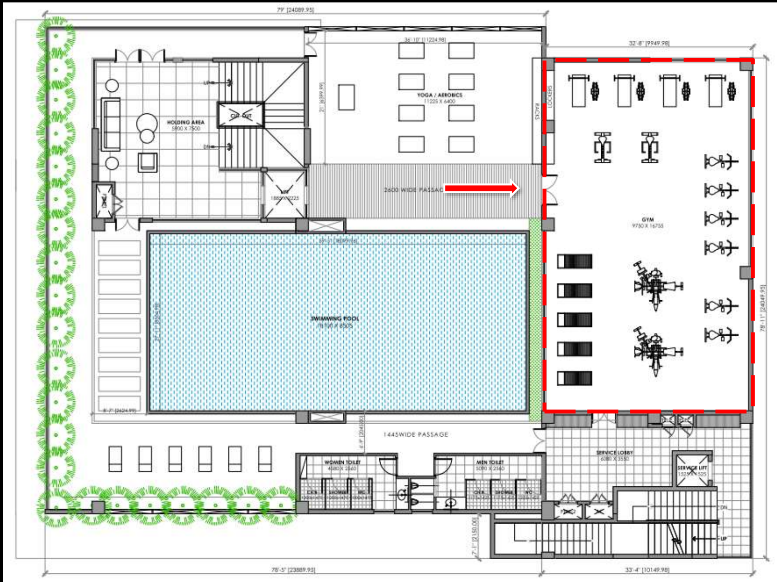
Fourth Floor plan – Gym area
