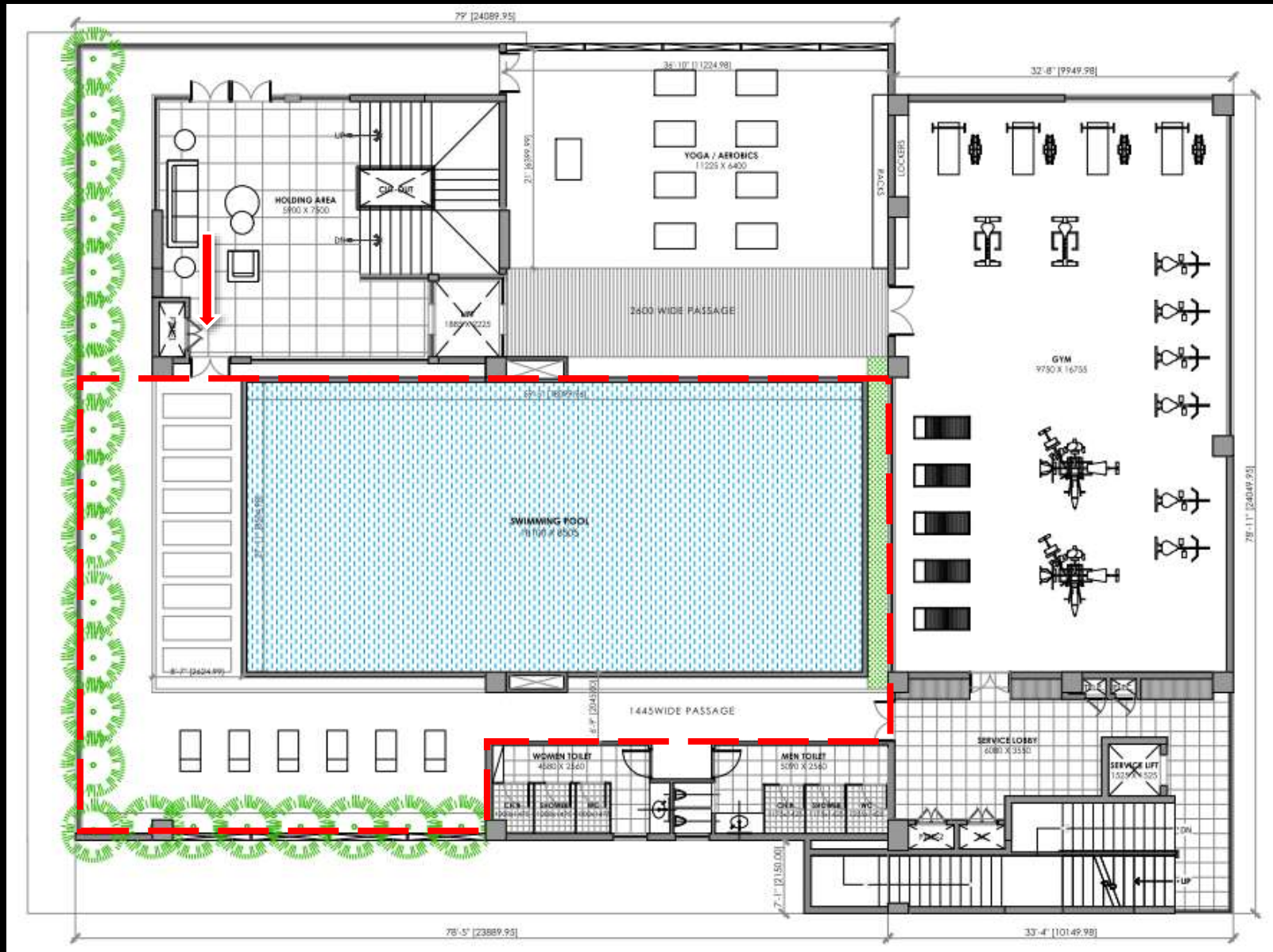
Fourth Floor plan – Pool area
