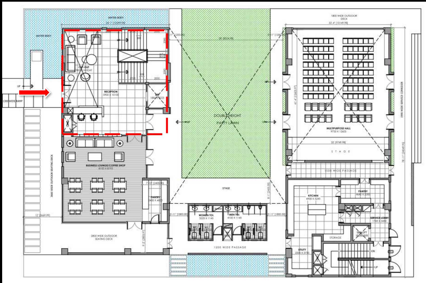
Ground Floor Plan - Entrance Lobby
